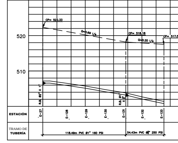
PERFIL LD – RAMAL 3 ESCALA HORIZONTAL 1:2,000 VERTICAL 1:400
