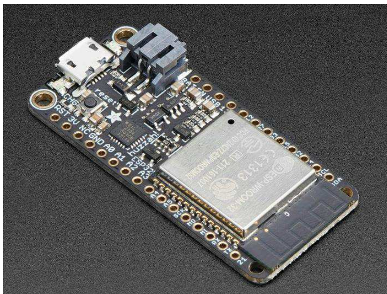
Figura 7. Adafruit HUZZAH32–ESP32 Feather Board
