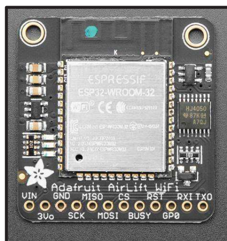
Figura 6. Adafruit AirLift WiFi ESP32
