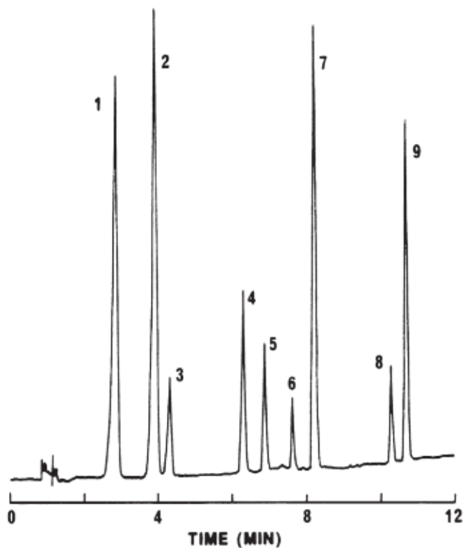
Figure 983.15. Chromatographic separation of antioxidant standards, ca 0.1 \mu g each antioxidant: 1, PG; 2, THBP; 3, TBHQ; 4, NDGA; 5, BHA; 6, Ionox-100; 7, OG; 8, BHT; 9, DG.
